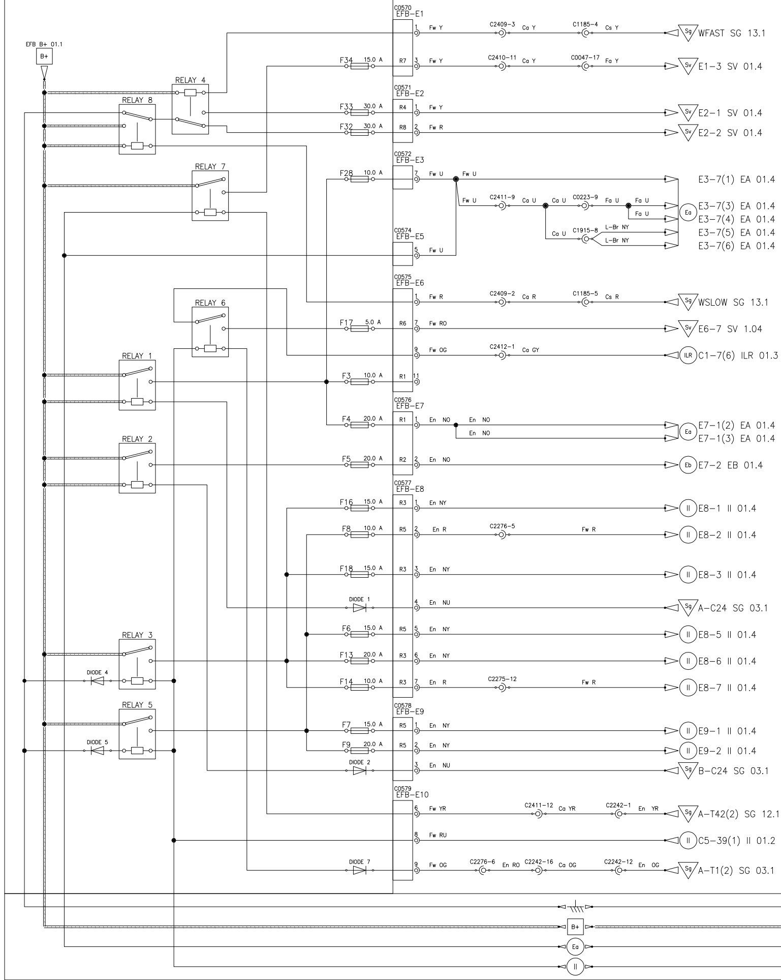
EFB (Engine Bay Fusebox) – Relays 1–8
