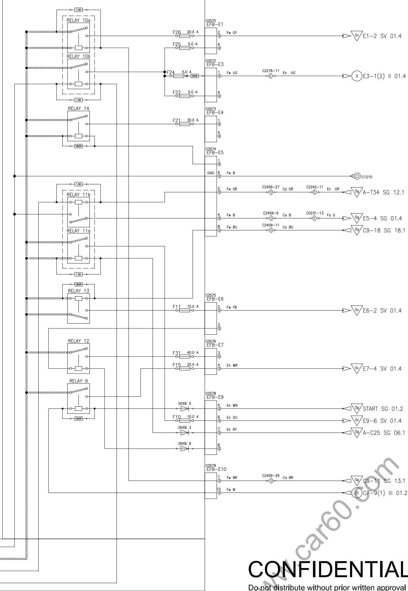
EFB (Engine Bay Fusebox) – Relays 9–14
